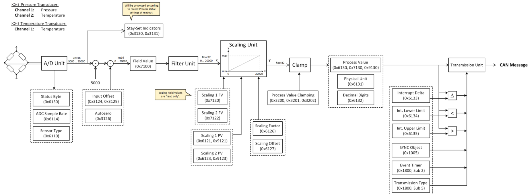
Figure 1: Data flow within the KD41 transducer
