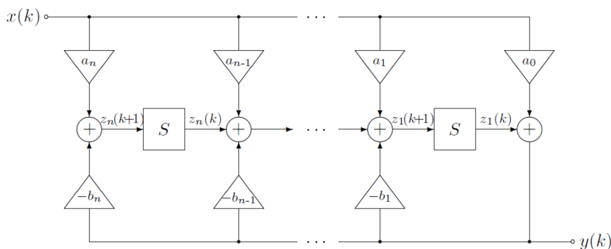
Figure 2: 5-Stage IIR Filter Unit
