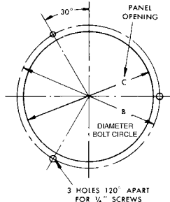
PANEL MOUNTING
