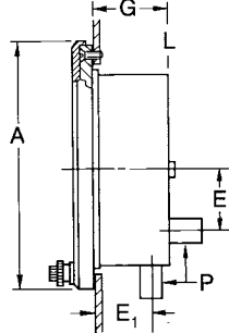
PANEL MOUNTING
