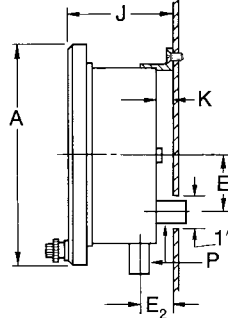
WALL MOUNTING
