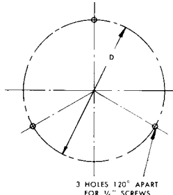
WALL MOUNTING
